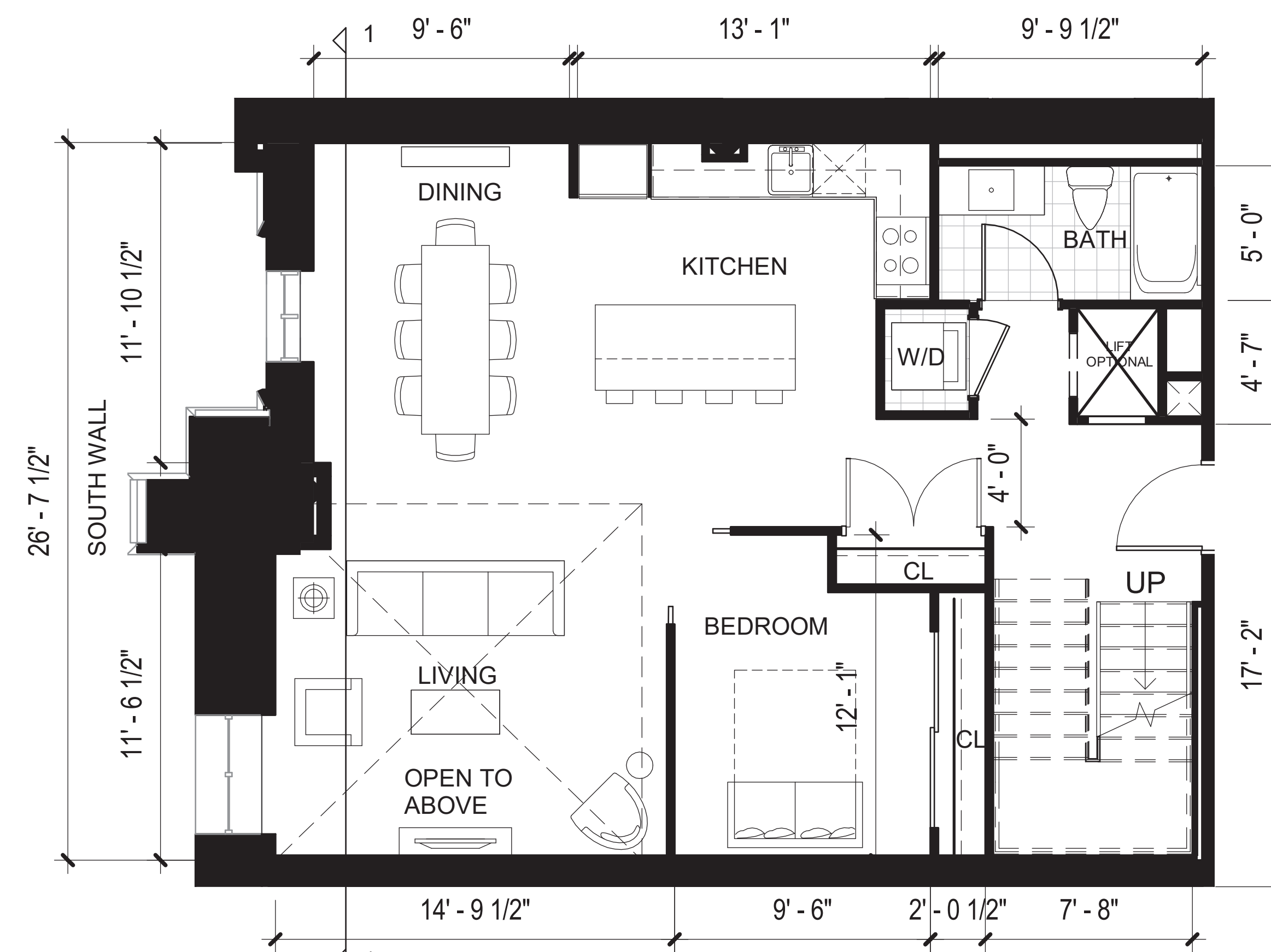
LOWER LEVEL PLAN
